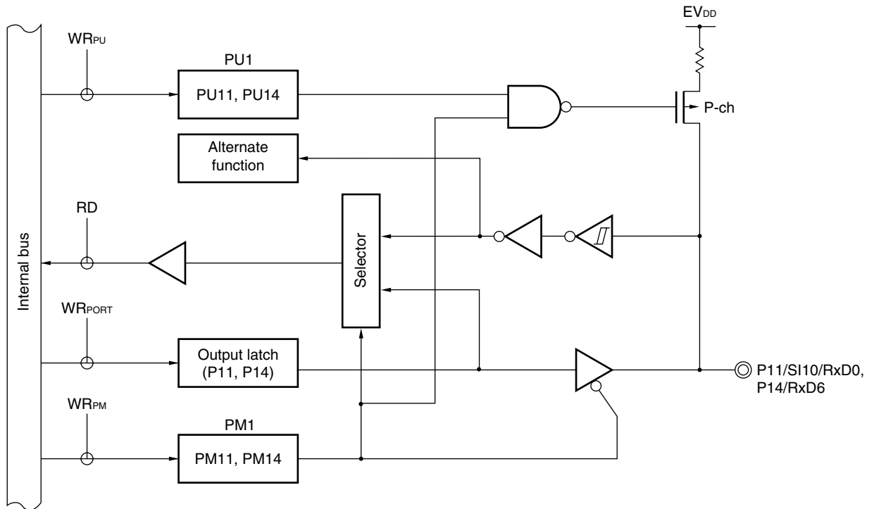
Figure 4-7. Block Diagram of P11 and P14
