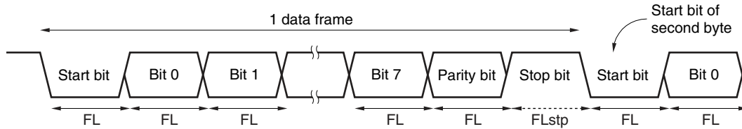
Figure 14-27. Data Frame Length During Continuous Transmission
