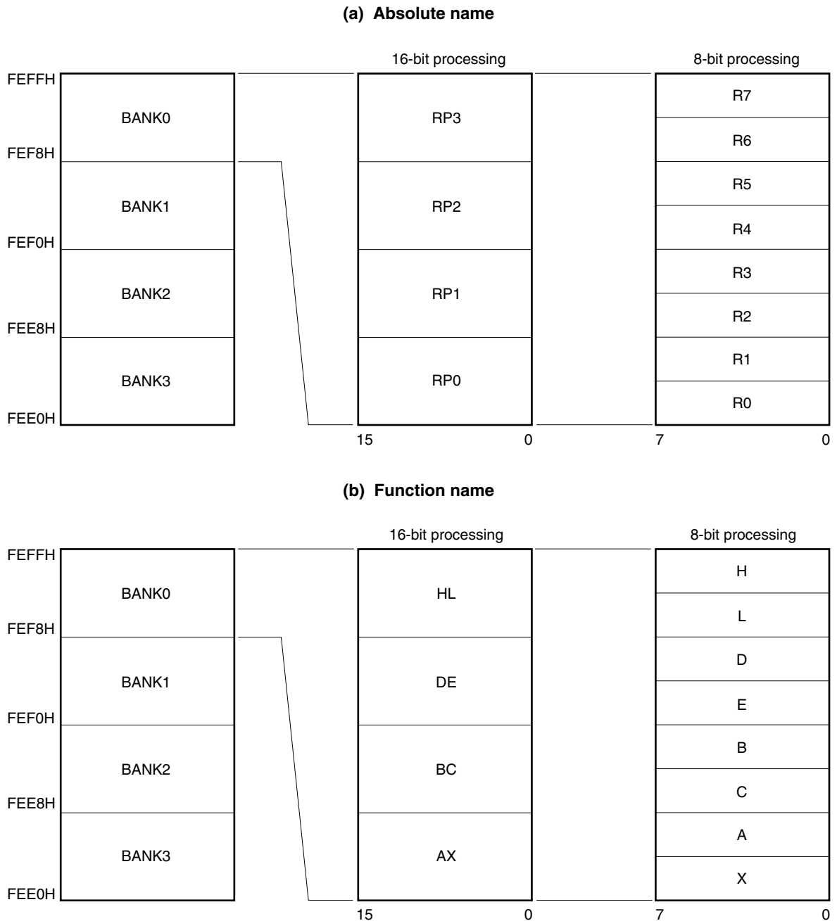
Figure 3-22. Configuration of General-Purpose Registers
