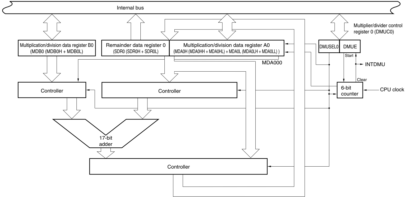
Figure 16-1. Block Diagram of Multiplier/Divider
