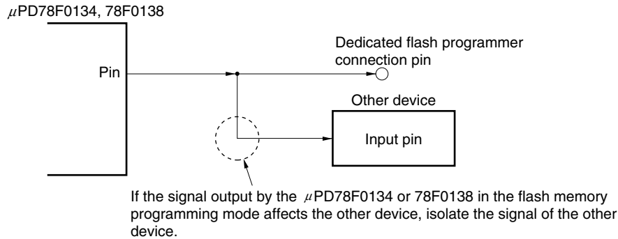
Figure 27-16. Malfunction of Other Device
