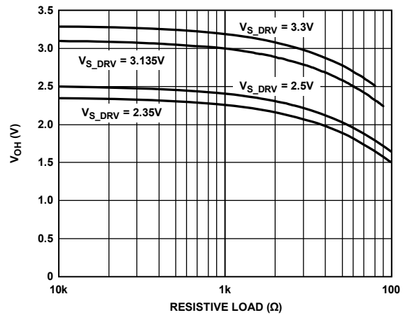
Figure 15. CMOS Output V_{OH} (Static) vs. R_{LOAD} (to Ground)
