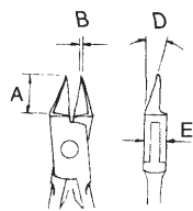
Head Dimensions: A-.55" B-.05" D-13° E-.28"
