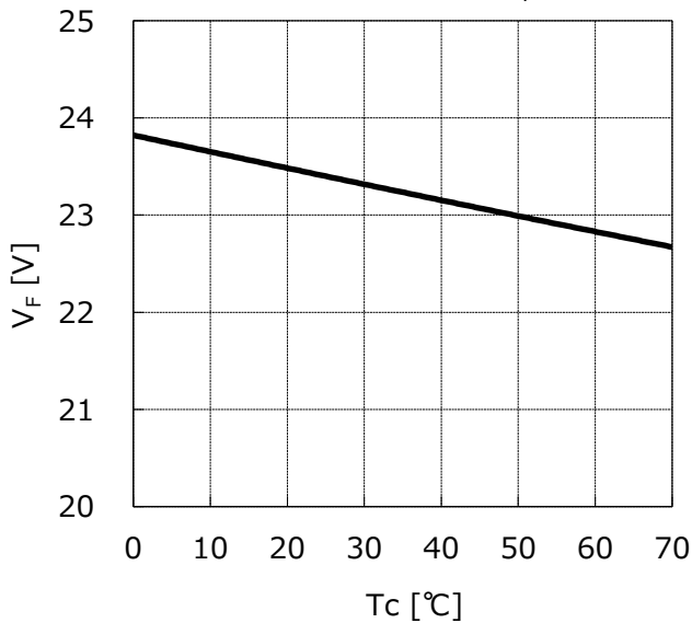
◆ T_c Temperature – Forward Voltage Characteristics I_F = 250\text{mA}
