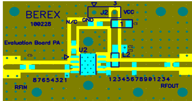
PCB Mounting
