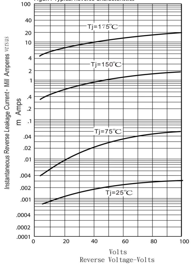
Figur.4-Typical Reverse Characteristics
