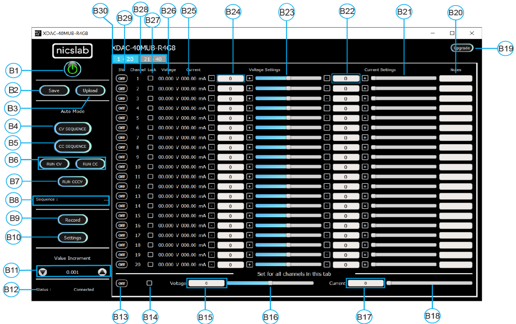
Figure 4. GUI
