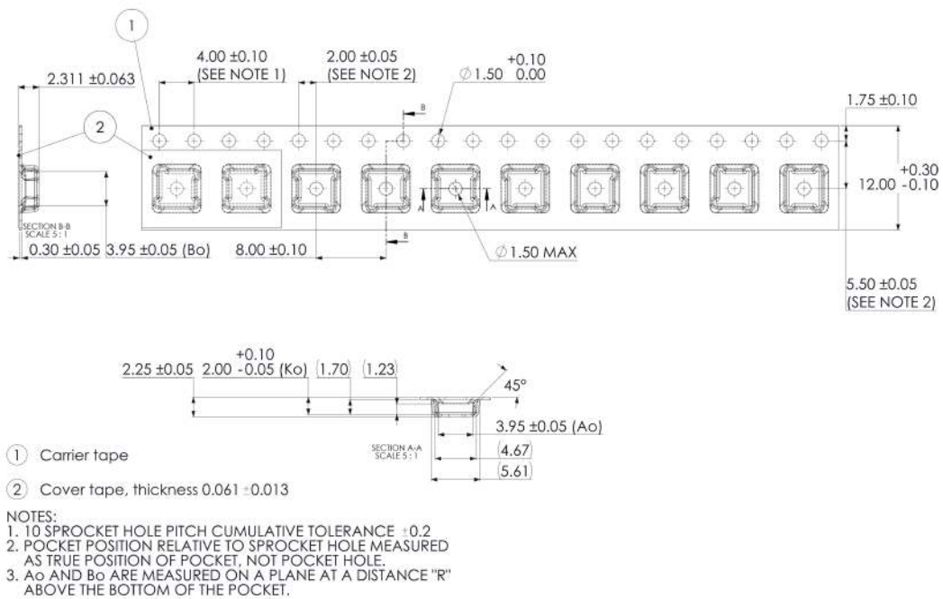
Figure 14d. Pocket tape dimensions for L110-Axxx145020000 and L110-Axxx150000000
