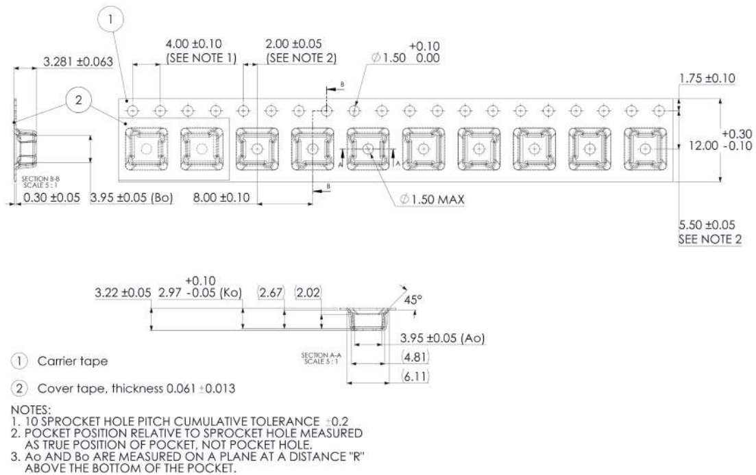
Figure 14c. Pocket tape dimensions for L110-Axxx090020000
