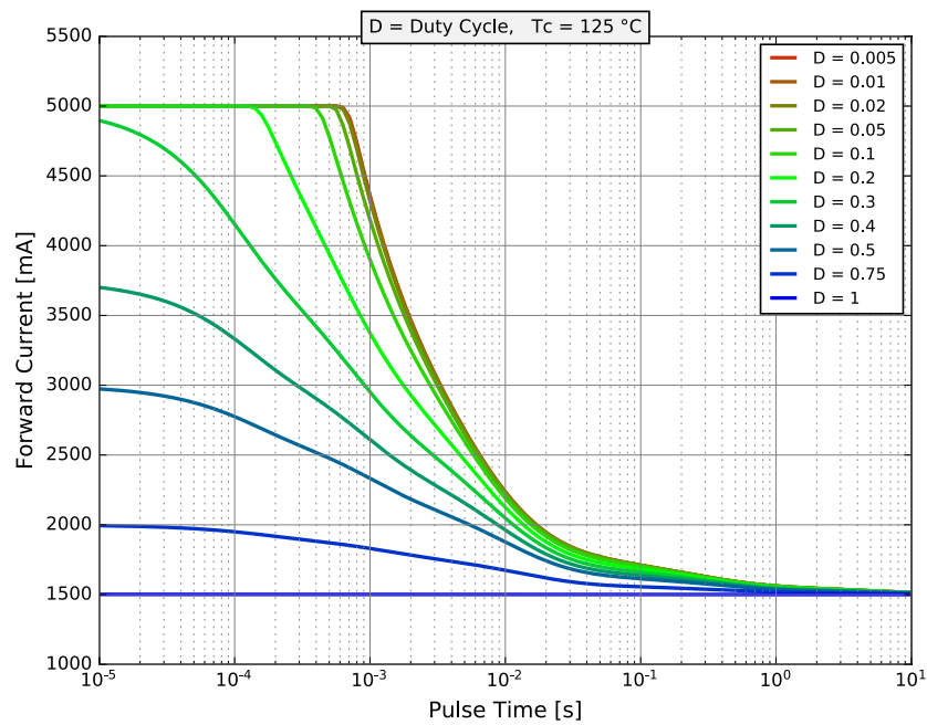
Figure 11. Permissible pulse handling capability for LUXEON IR Domed Gen 2 at T_c = up to 125\text{ °C}
