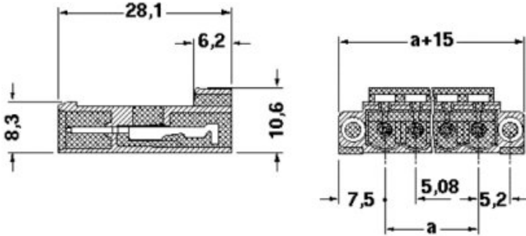
Dimensioned drawing
