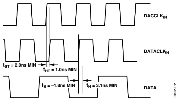
Figure 52. Low Setup and Hold Mode Timing, 1x Interpolation, DCLKPOL = 1
