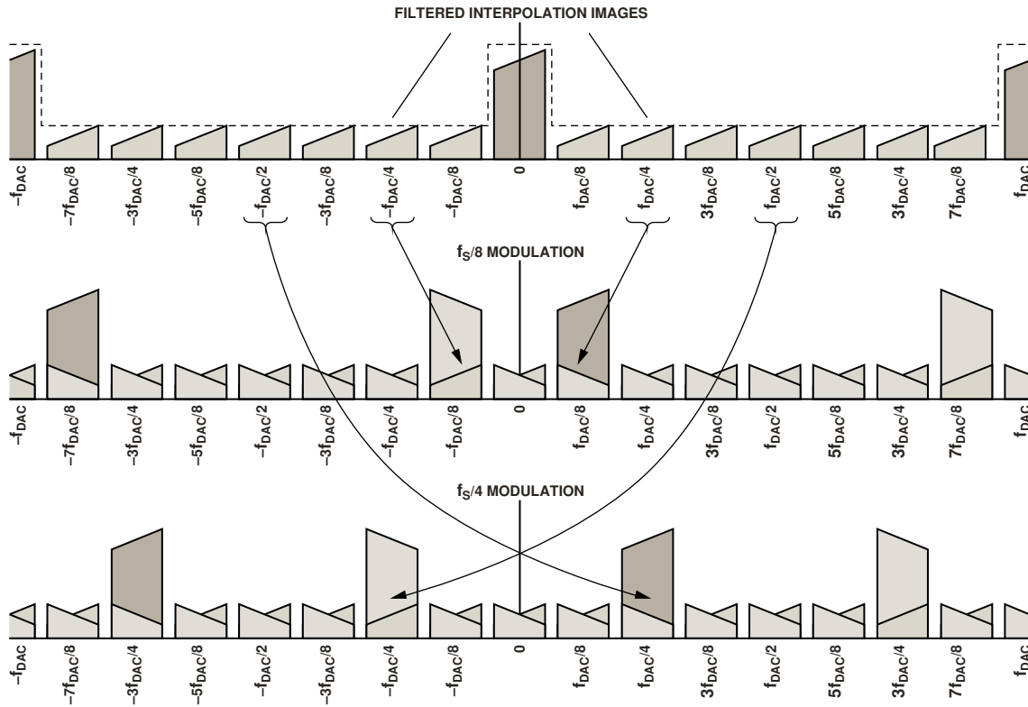
Figure 70. Complex Modulation with Negative Frequency Aliasing
