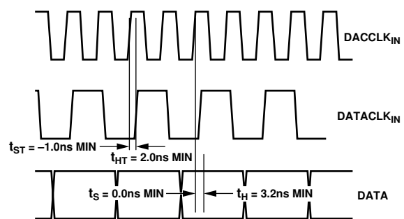
Figure 50. Slave Mode Timing, 2x Interpolation, DCLKPOL = 1
