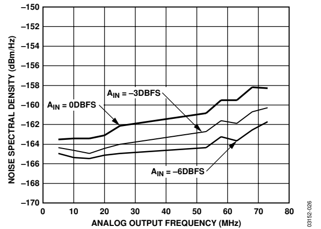
Figure 26. Noise Spectral Density vs. Analog Input Frequency, f_{DATA} = 78 MSPS, 2x Interpolation
