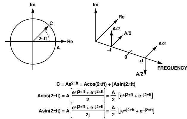
Figure 58. Complex Phasor Representation
