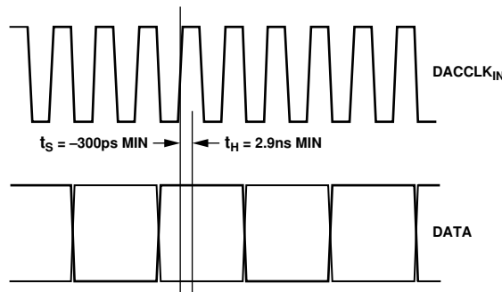
Figure 53. External Sync Mode with 2x Interpolation
