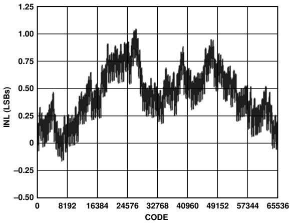
Figure 22. Typical INL
