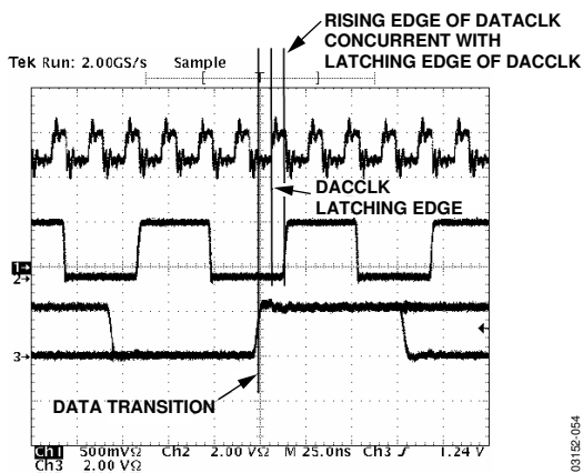
Figure 54. DATAADJ = 0000
