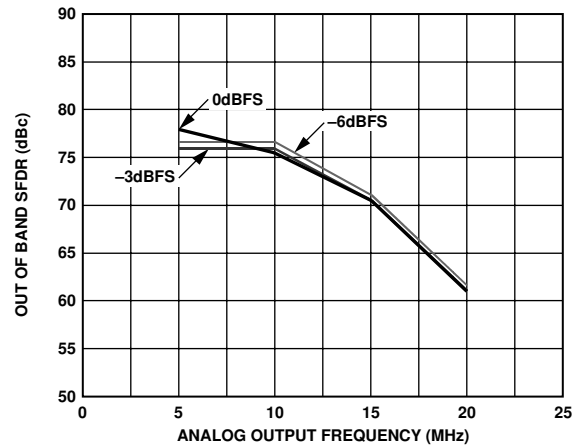
Figure 13. Out-of-Band SFDR, f_{DATA} = 50 MSPS, 8x Interpolation
