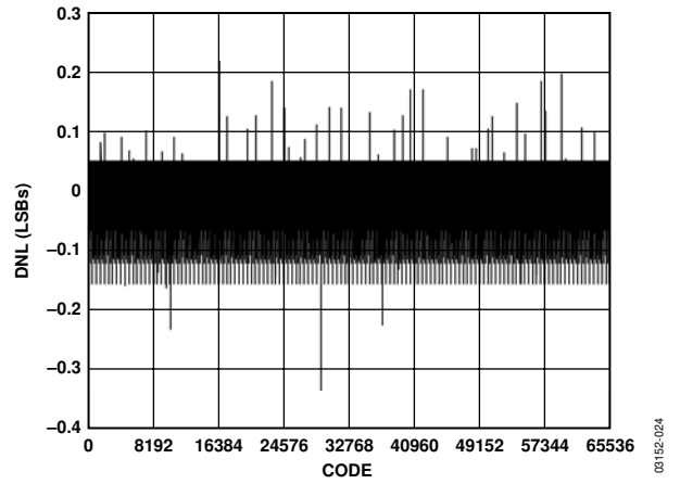
Figure 24. Typical DNL
