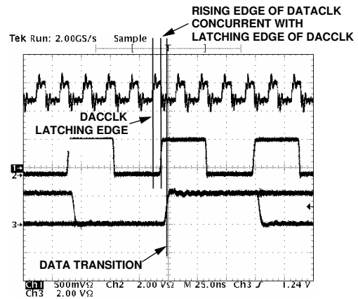
Figure 55. DATAADJ = 1111
