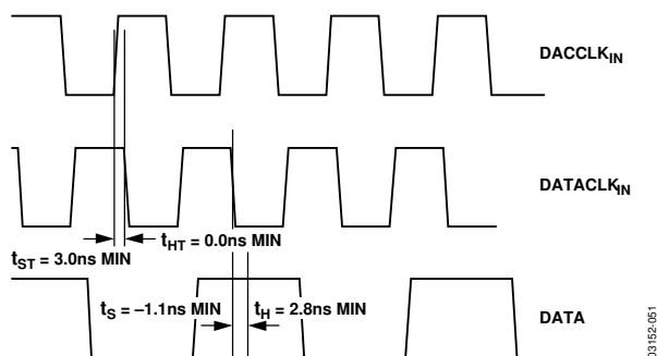
Figure 51. Low Setup and Hold Mode Timing, 1x Interpolation, DCLKPOL = 0
