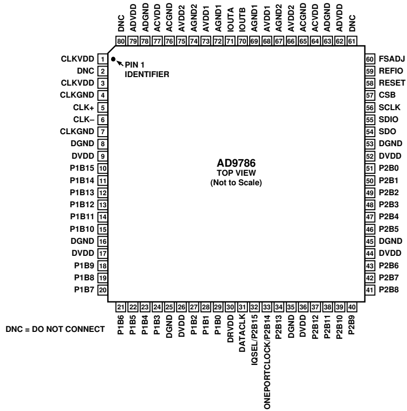
Figure 2. Pin Configuration
