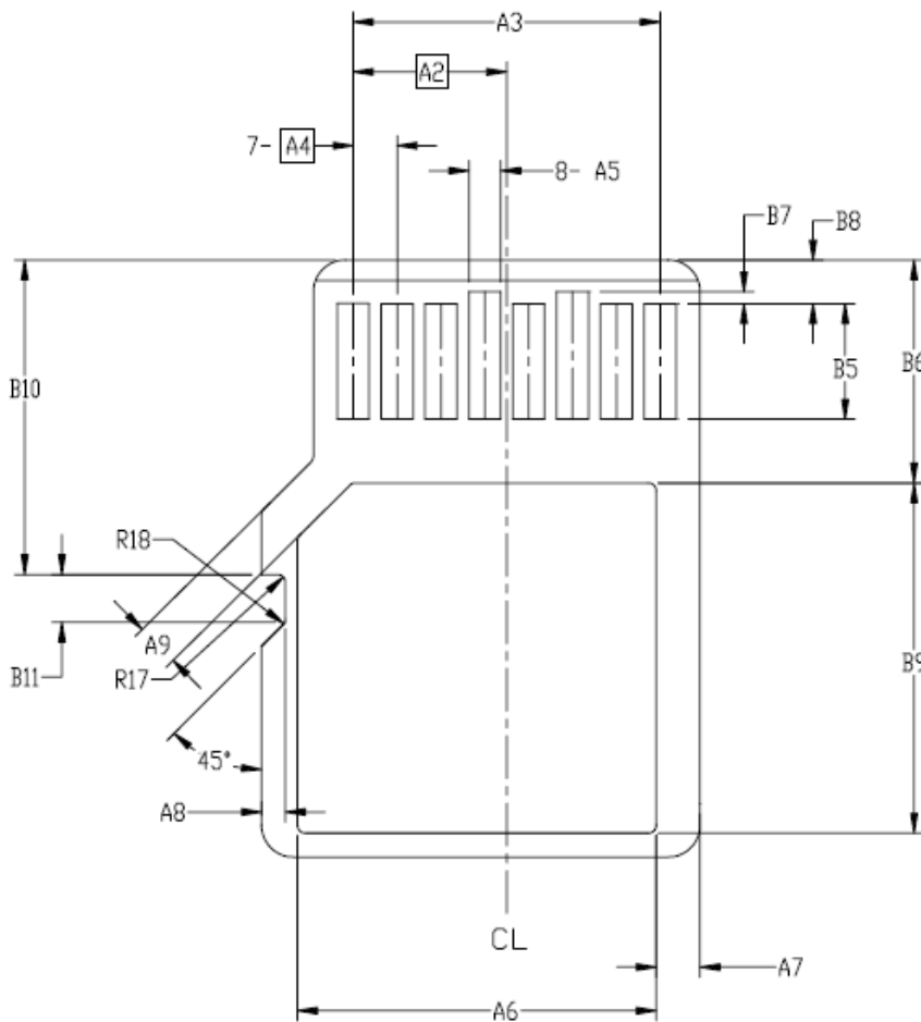
Figure 3-15 -1 Dimensions of microSD (Bottom View)
