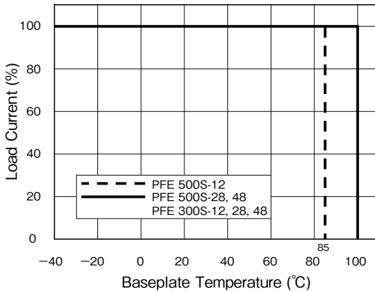
Fig. 12-2 Derating Curve
