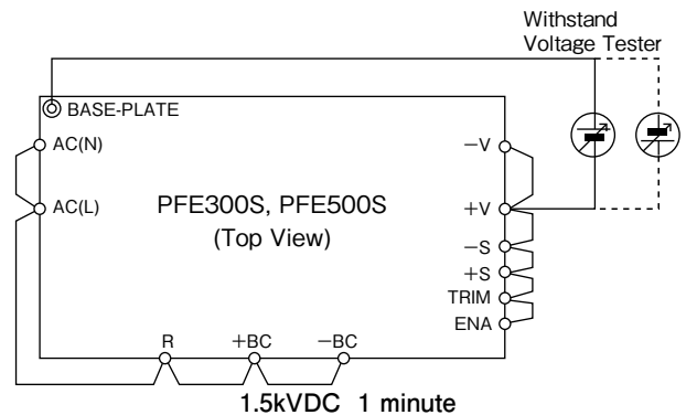
Fig.17-3 Output to Baseplate Withstand Voltage Test Method
