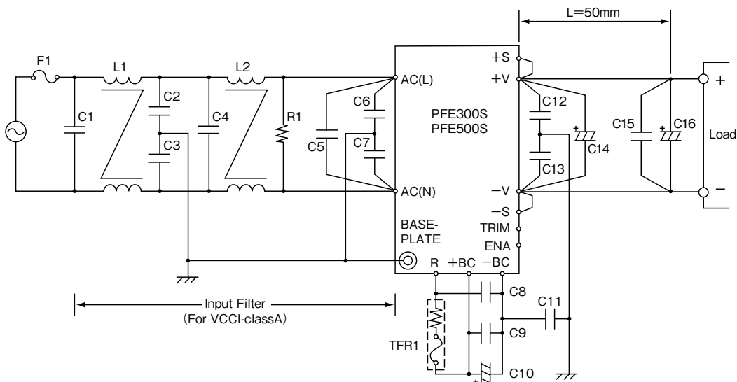
Fig. 1-1 Basic Connection
