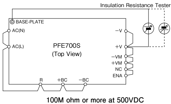
Fig. 17-1 Insulation Resistance Test Method
