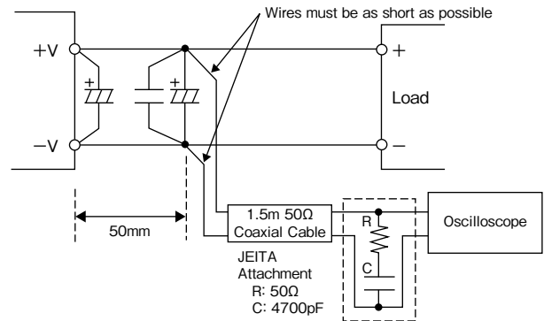
Fig. 3-1 Output Ripple Voltage (including Spike Noise) Measurement Method
