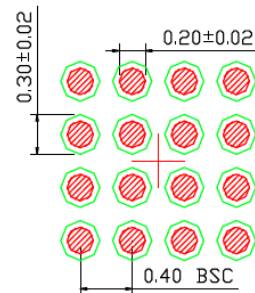
RECOMMENDED LAND PATTERN NOTE: 3, 4
