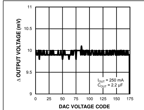
FIGURE 2-16: Δ Output Voltage vs. DAC DNL.
