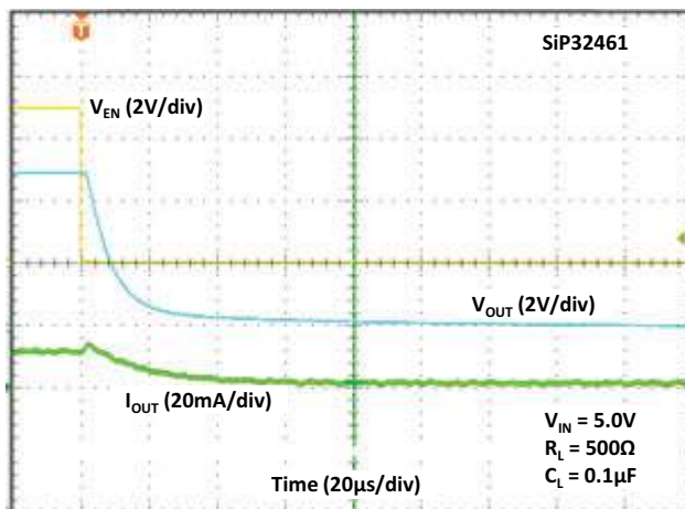
Fig. 40 - Turn-off Time
