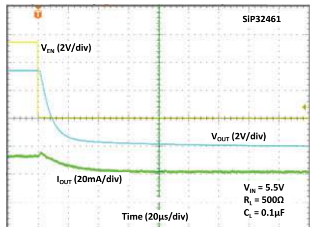
Fig. 43 - Turn-off Time
