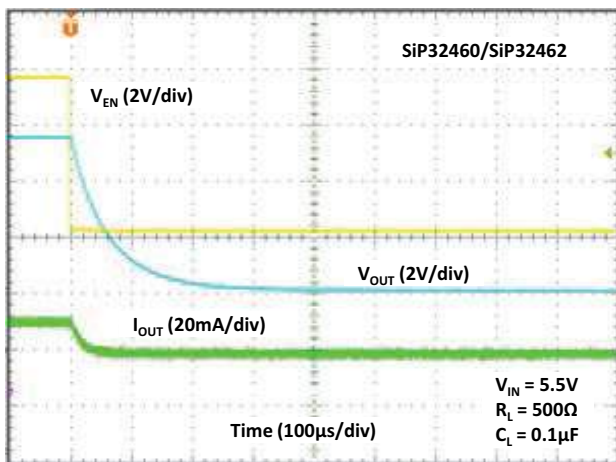
Fig. 39 - Turn-off Time
