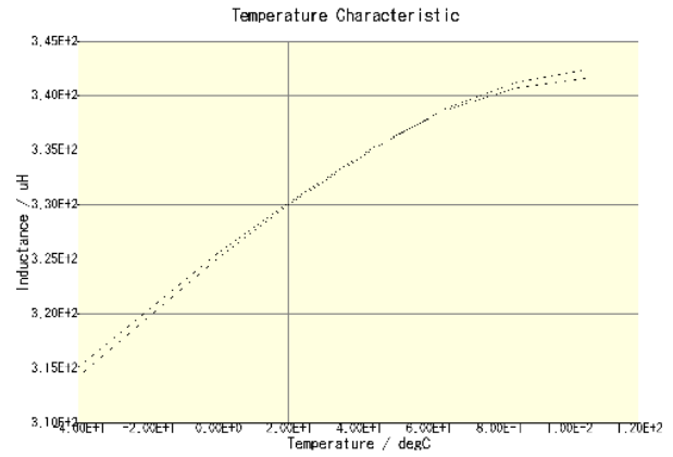
CLF12555T-331M-CA(DC = 0A)
