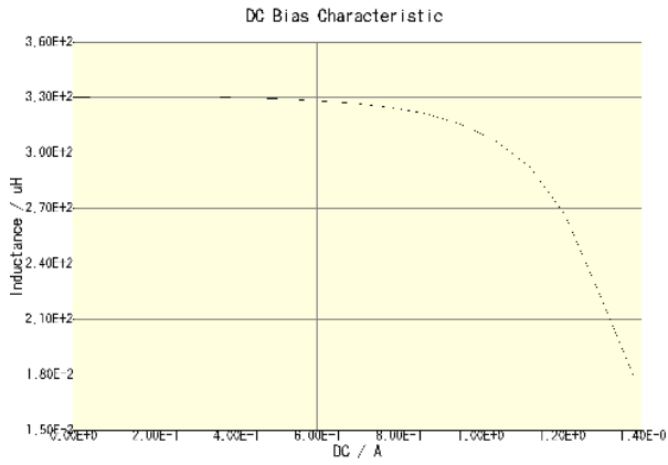
CLF12555T-331M-CA(Amb. Temp. = 20degC)
