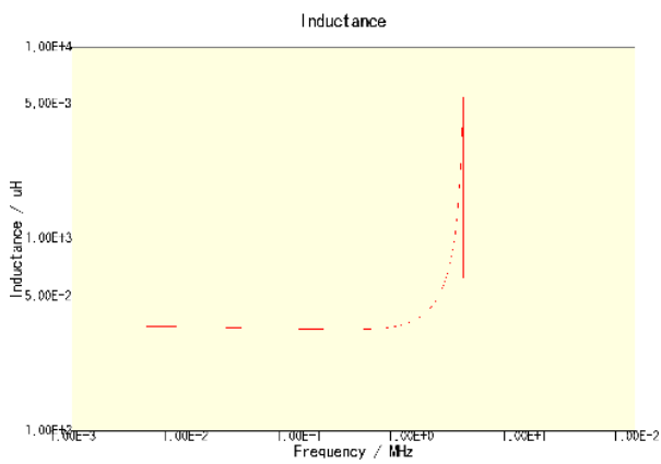
CLF12555T-331M-CA
