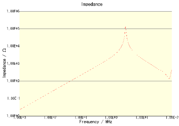
CLF12555T-331M-CA
