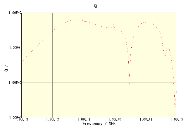
CLF12555T-331M-CA
