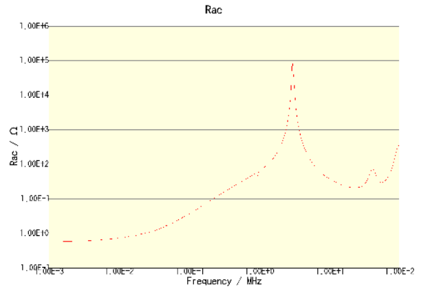
CLF12555T-331M-CA
