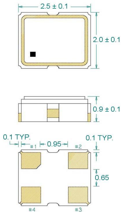
Bottom View
