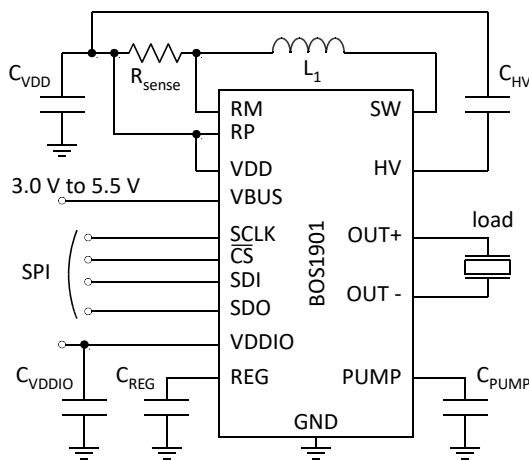
Figure 1: Simplified schematic
