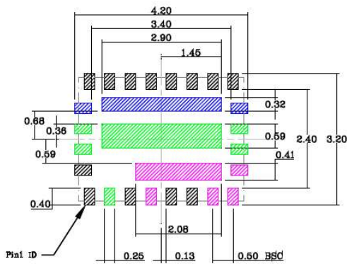
Solder Stencil Opening
