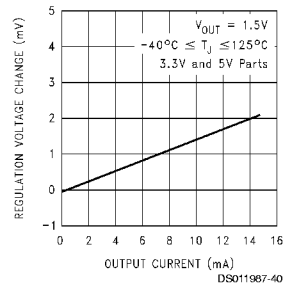
Regulation Voltage Change vs Output Current
