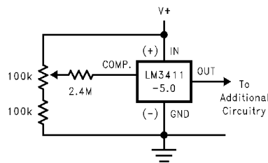
FIGURE 13. \pm 50 mV External Trim
