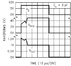
Response Time for 5V Version ( C_C = 0 pF)
