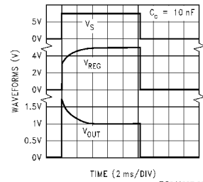
Response Time for 5V Version ( C_C = 10 nF)
