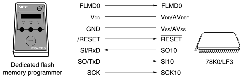
Figure 28-6. Communication with Dedicated Flash memory programmer (CSI10)
