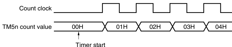
Figure 7-20. 8-Bit Timer Counter 5n Start Timing
