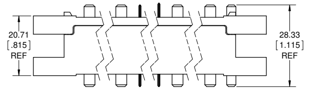
PIN AND SOCKET MATED ASSEMBLY
