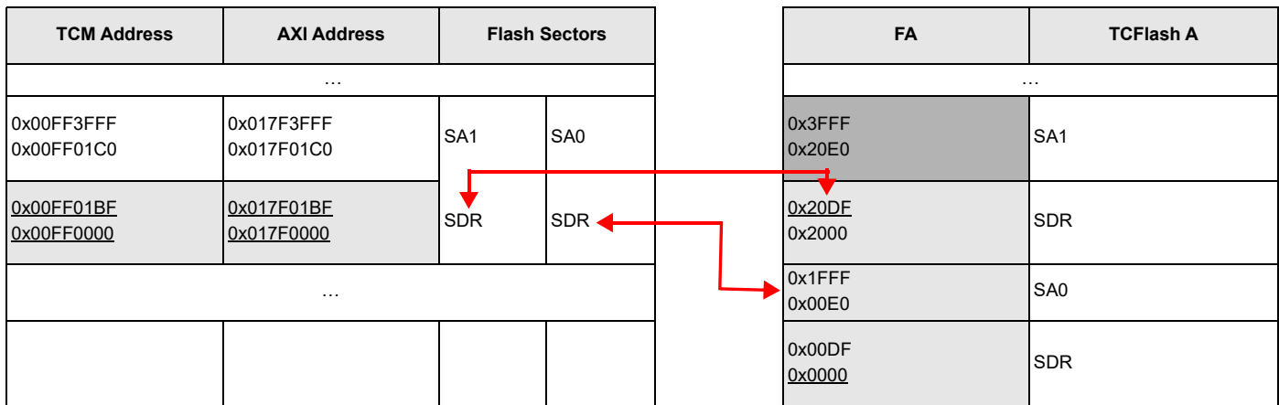
Interleaved arrangement of Flash sectors in CPU Address Map
