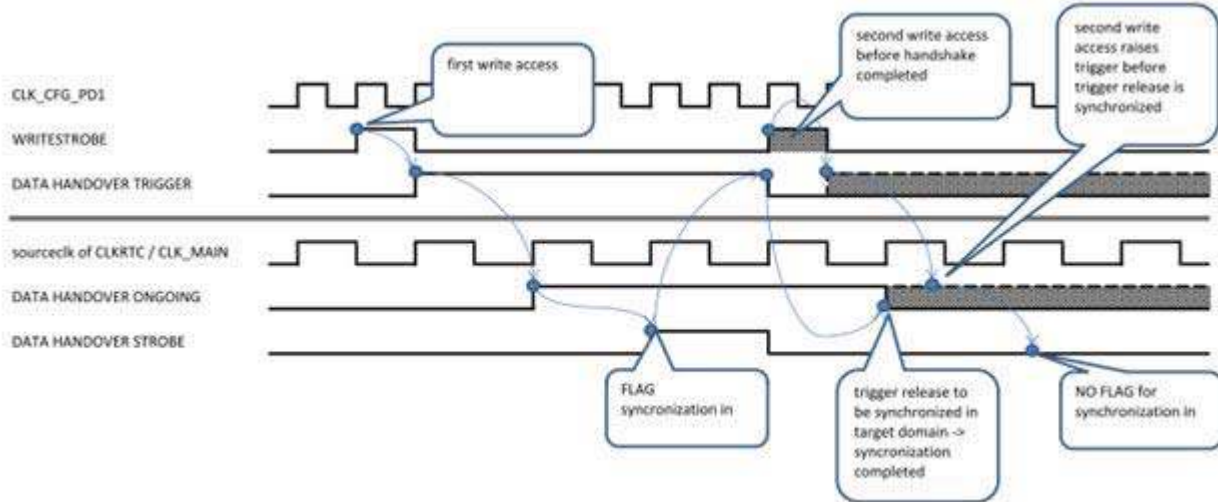
Figure 29. Handshake Synchronization
