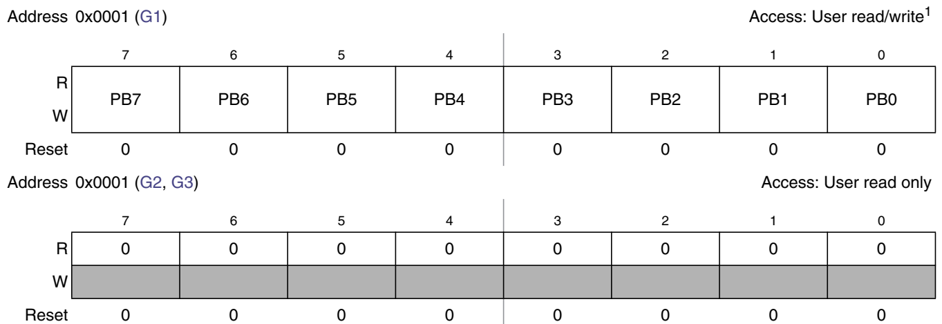
Figure 2-3. Port B Data Register (PORTB)
