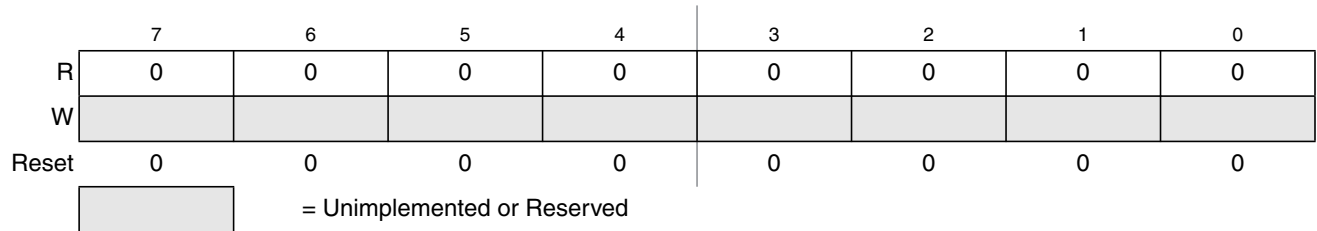
Figure 29-8. Flash Reserved0 Register (FRSV0)
