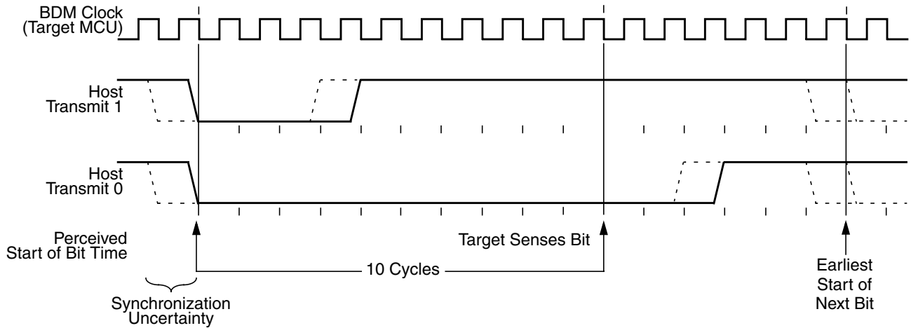
Figure 7-7. BDM Host-to-Target Serial Bit Timing
