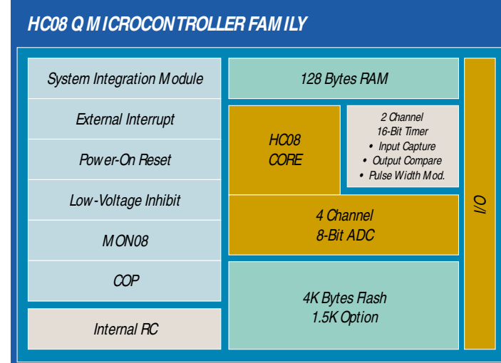
The HC08 Q family includes six devices based on the HC08 architecture: the 8-pin 68HC908QT1, 68HC908QT2 and 68HC908QT4; and the 16-pin 68HC908QY1, 68HC908QY2 and 68HC908QY4.
