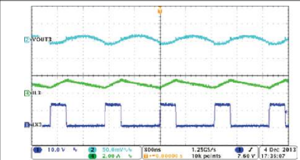
Figure 8-14. Buck3, Steady State Operation With Full Load
