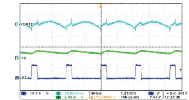
Figure 8-12. Buck2, Steady State Operation With Full Load
