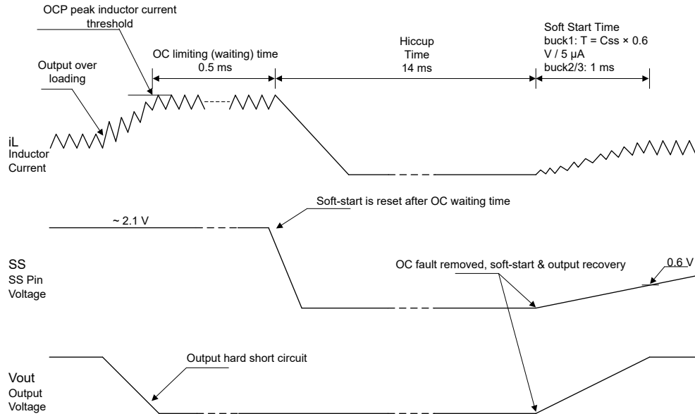
Figure 7-7. Overcurrent Protection
