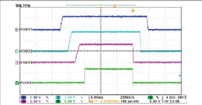
Figure 8-28. Automatic Power Sequencing, MODE = EN1 = EN2 = HIGH
