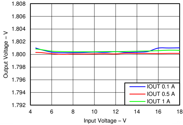
Figure 6-7. Buck2, Line Regulation
