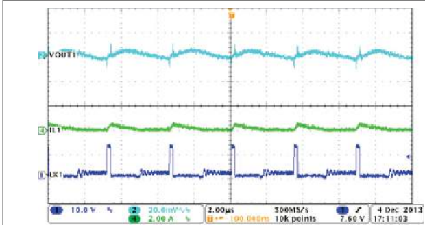
Figure 8-9. Buck1, Steady State Operation With Light Load
