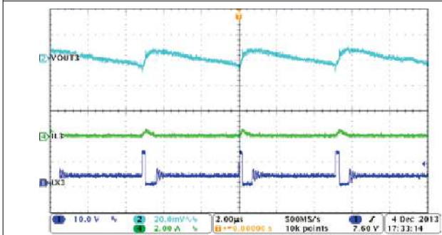
Figure 8-13. Buck3, Steady State Operation With Light Load
