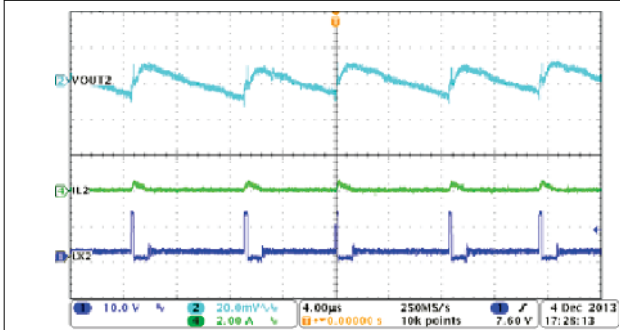
Figure 8-11. Buck2, Steady State Operation With Light Load
