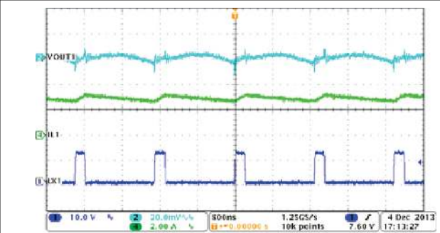
Figure 8-10. Buck1, Steady State Operation With Full Load
