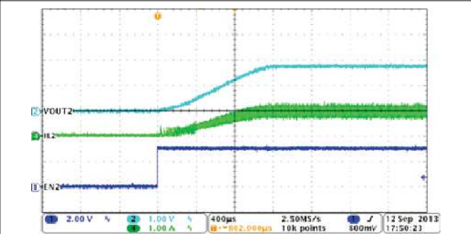
Figure 8-6. Buck2, Soft-Start With Full Load
