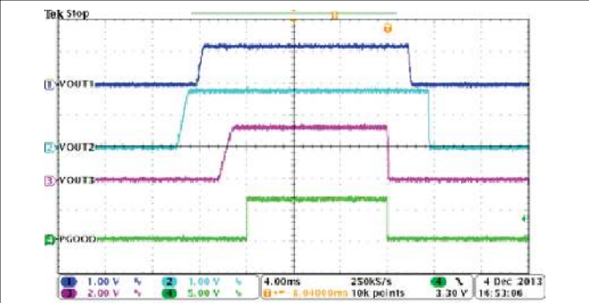
Figure 8-32. Automatic Power Sequencing, MODE = EN2 = HIGH, EN1 = LOW
