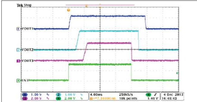
Figure 8-27. Automatic Power Sequencing, MODE = EN1 = EN2 = HIGH
