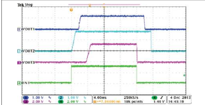
Figure 8-31. Automatic Power Sequencing, MODE = EN2 = HIGH, EN1 = LOW
