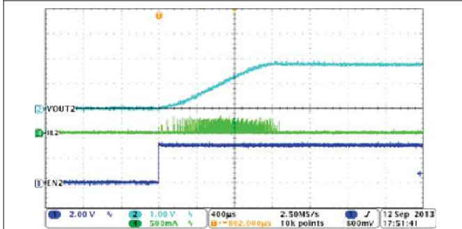
Figure 8-5. Buck2, Soft-Start With No Load
