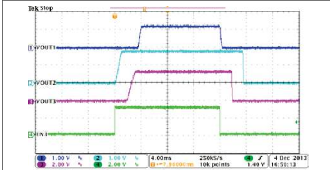
Figure 8-29. Automatic Power Sequencing, MODE = EN1 = HIGH, EN2 = LOW
