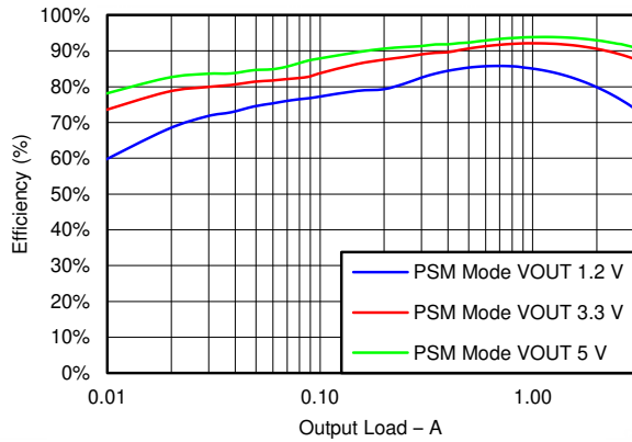
Figure 6-1. Buck1 Efficiency
