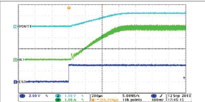
Figure 8-4. Buck1, Soft-Start With Full Load
