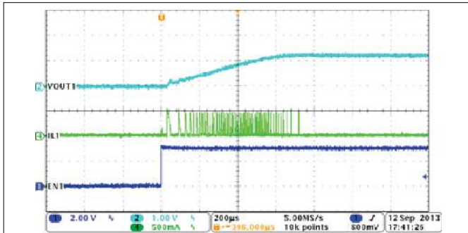
Figure 8-3. Buck1, Soft-Start With No Load
