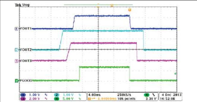
Figure 8-30. Automatic Power Sequencing, MODE = EN1 = HIGH, EN2 = LOW
