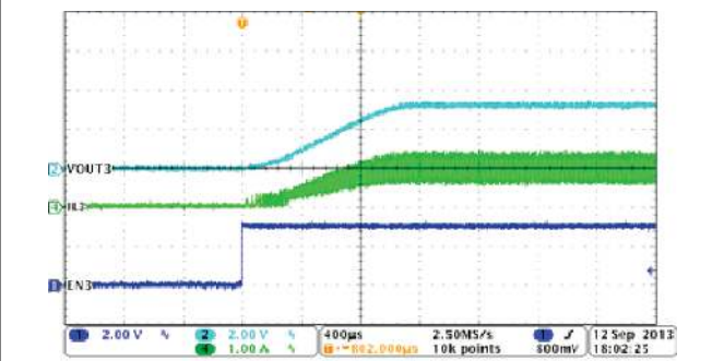
Figure 8-8. Buck3, Soft-Start With Full Load
