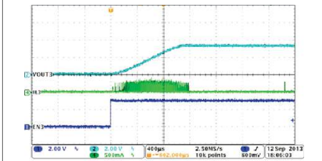
Figure 8-7. Buck3, Soft-Start With No Load
