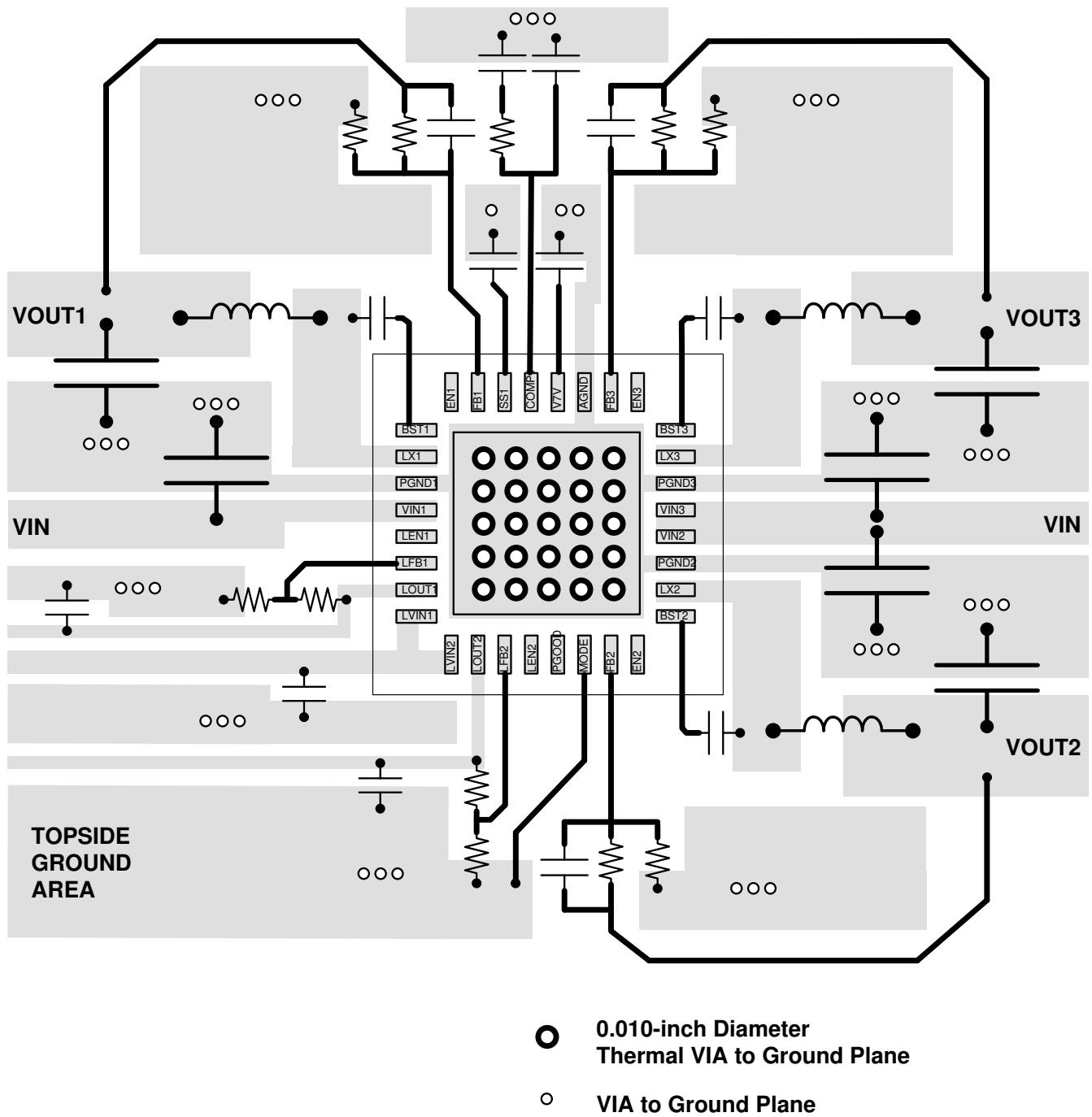
Figure 8-35. PCB Layout
