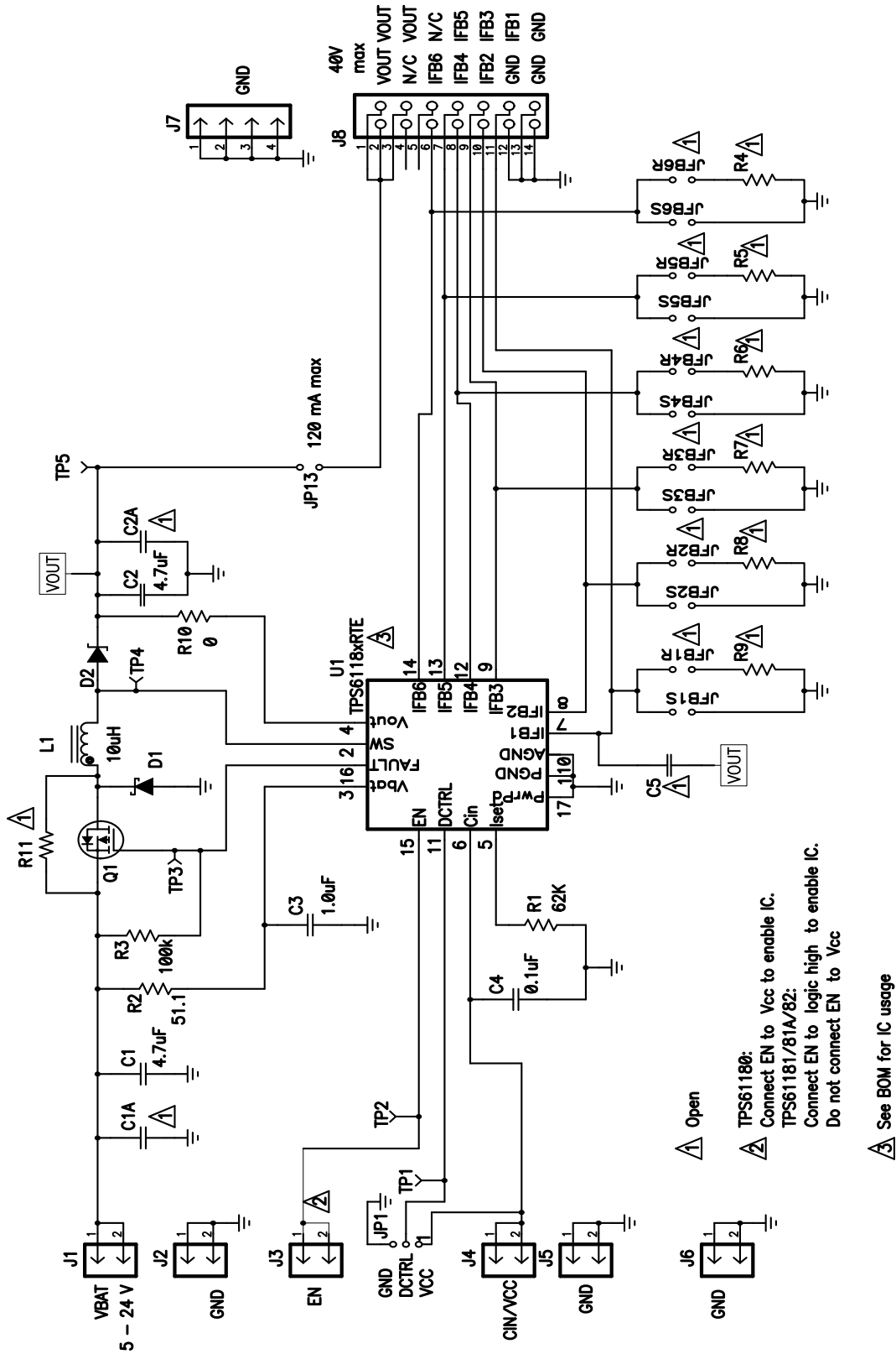
Figure 9. HPA259A Schematic
