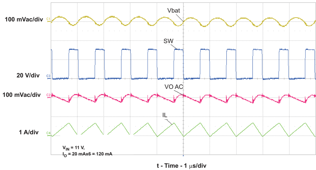
Figure 4. Switching Waveform
