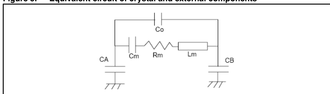
Figure 5. Equivalent circuit of crystal and external components
