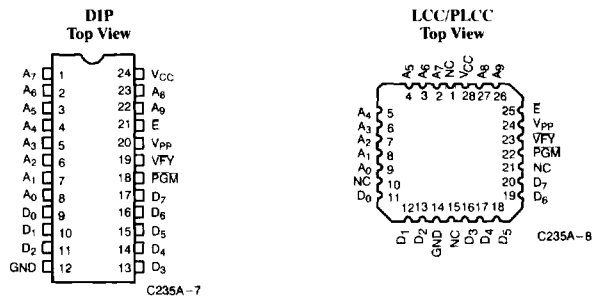
Figure 1. Programming Pinouts
