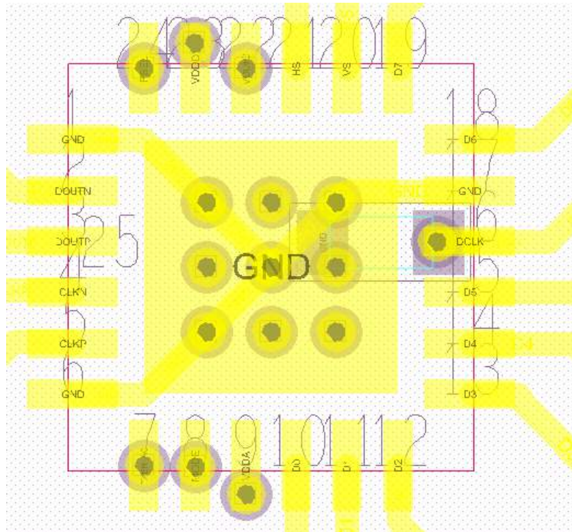
Figure 32. Footprint Example
