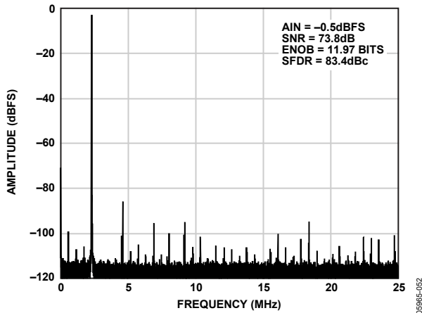
Figure 15. Single-Tone 32k FFT with f_{IN} = 2.4\text{ MHz} , f_{SAMPLE} = 50\text{ MSPS}
