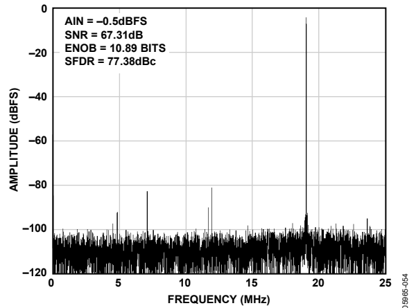
Figure 18. Single-Tone 32k FFT with f_{IN} = 170\text{ MHz} , f_{SAMPLE} = 50\text{ MSPS}
