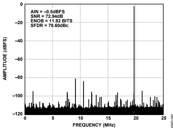
Figure 16. Single-Tone 32k FFT with f_{IN} = 70\text{ MHz} , f_{SAMPLE} = 50\text{ MSPS}
