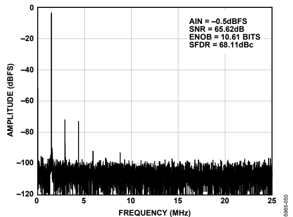
Figure 20. Single-Tone 32k FFT with f_{IN} = 250\text{ MHz} , f_{SAMPLE} = 50\text{ MSPS}
