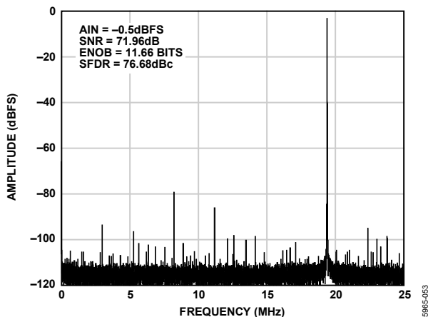
Figure 17. Single-Tone 32k FFT with f_{IN} = 120\text{ MHz} , f_{SAMPLE} = 50\text{ MSPS}
