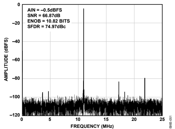
Figure 19. Single-Tone 32k FFT with f_{IN} = 190\text{ MHz} , f_{SAMPLE} = 50\text{ MSPS}
