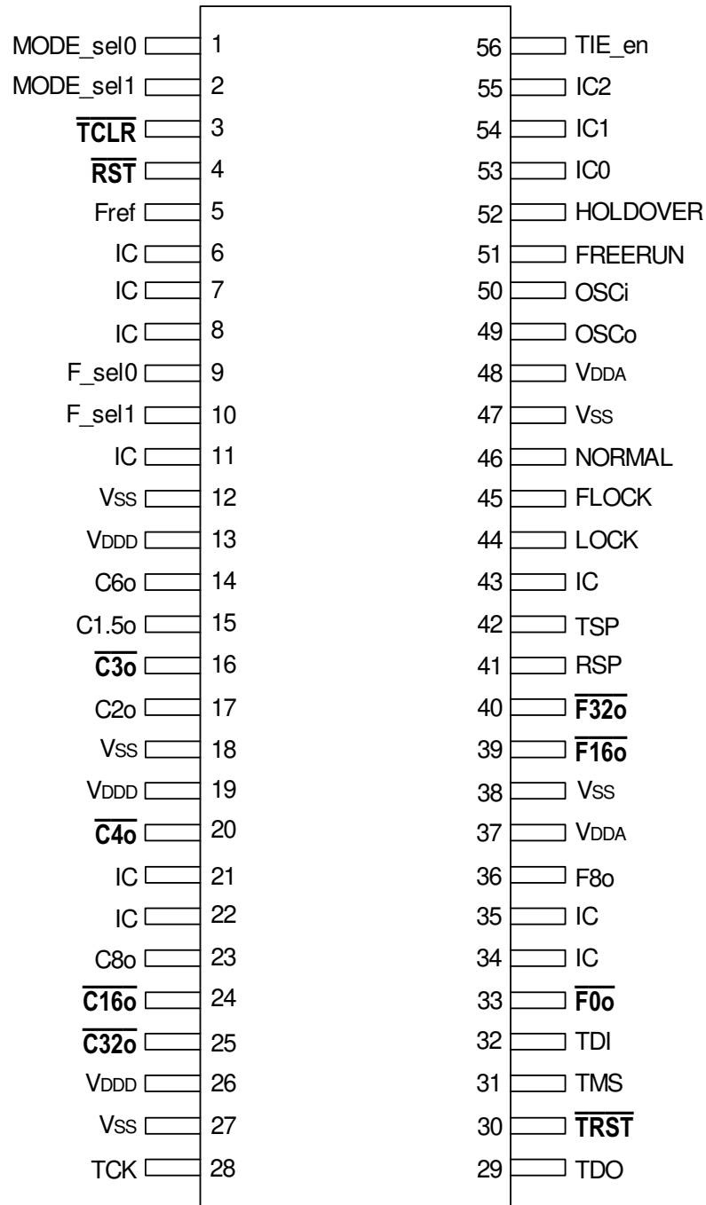
Figure - 2 IDT82V3001A SSOP56 Package Pin Assignment
