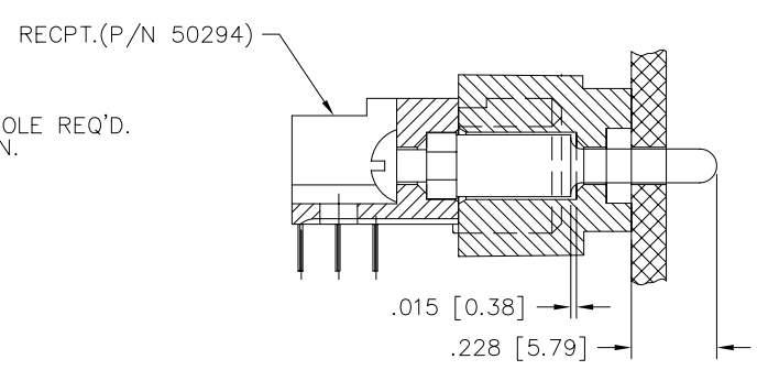
HOUSING FULLY MATED
