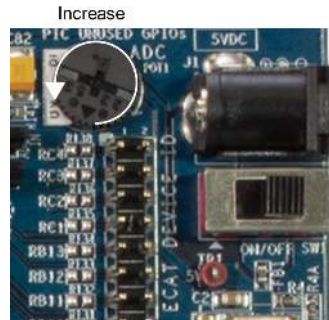
FIGURE 2-8: POTENTIOMETER POT1
