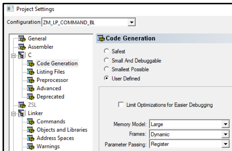
Figure 9. Code Generation
