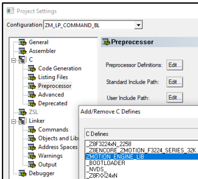
Figure 10. Preprocessor Definitions
