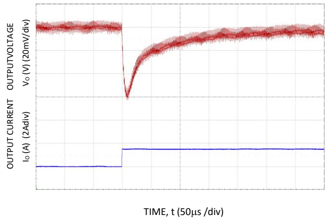
Figure 28. Transient Response to Dynamic Load Change from 50% to 100% at 12Vin, C out -2x100μF, Ctune-1nF, Rtune-500
