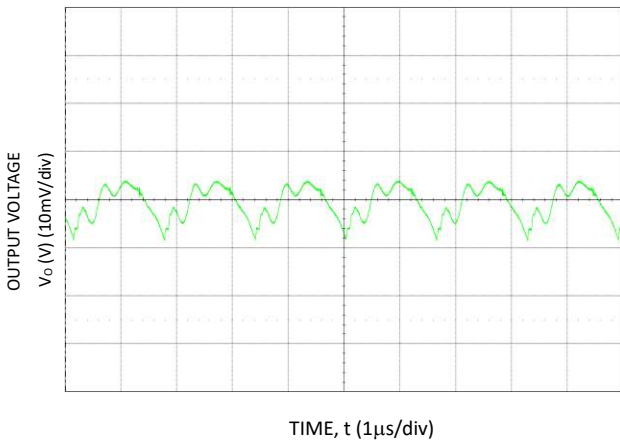
Figure 27. Typical output ripple and noise (C o =88μF ceramic, V IN = 12V, I o = I o,max ).
