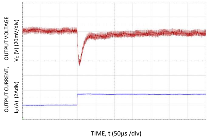
Figure 22. Transient Response to Dynamic Load Change from 50% to 100% at 12Vin, C_{out}=2 \times 100\mu\text{F} , C_{tune}=1.5\text{nF} , R_{tune}=500
