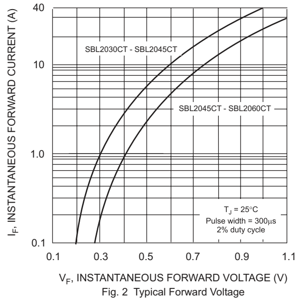
Fig. 2 Typical Forward Voltage
