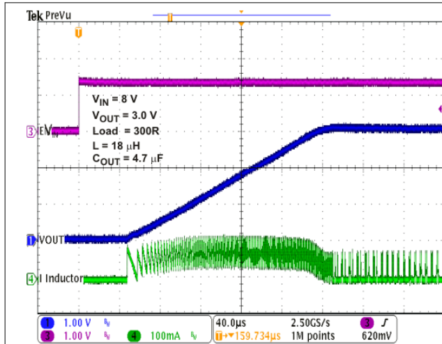
Figure 5-2. TPS62120EVM Start-up into 300- \Omega Load ( V_{IN} = 8.0\text{ V} , V_{OUT} = 3.0\text{ V} )
