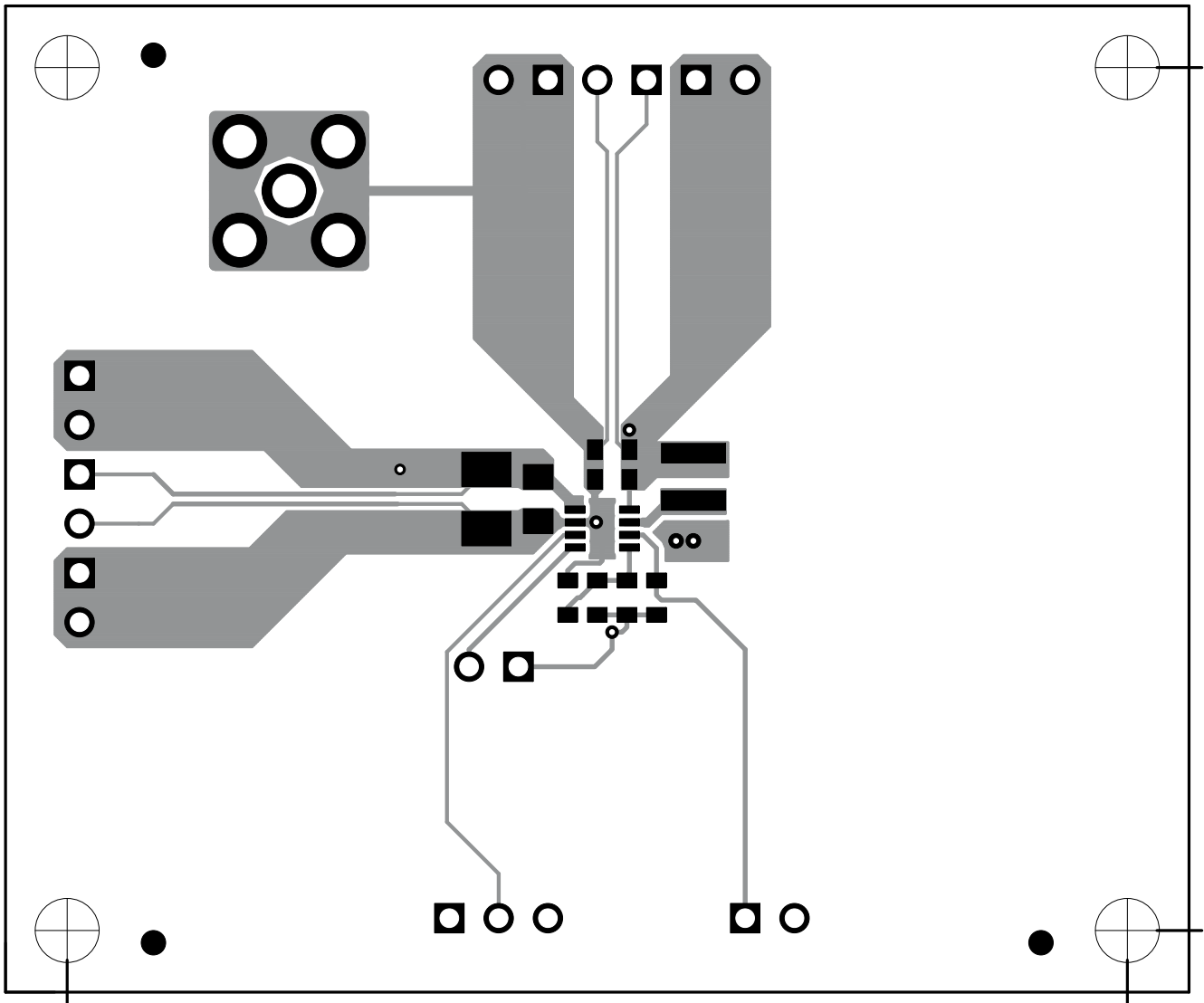
Figure 6-2. TPS62120EVM Top-Side Copper (Top View)
