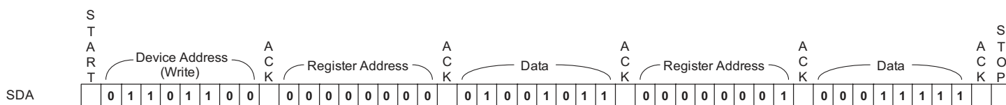
Figure 5: I 2 C Transfer Protocol for Example 1.
