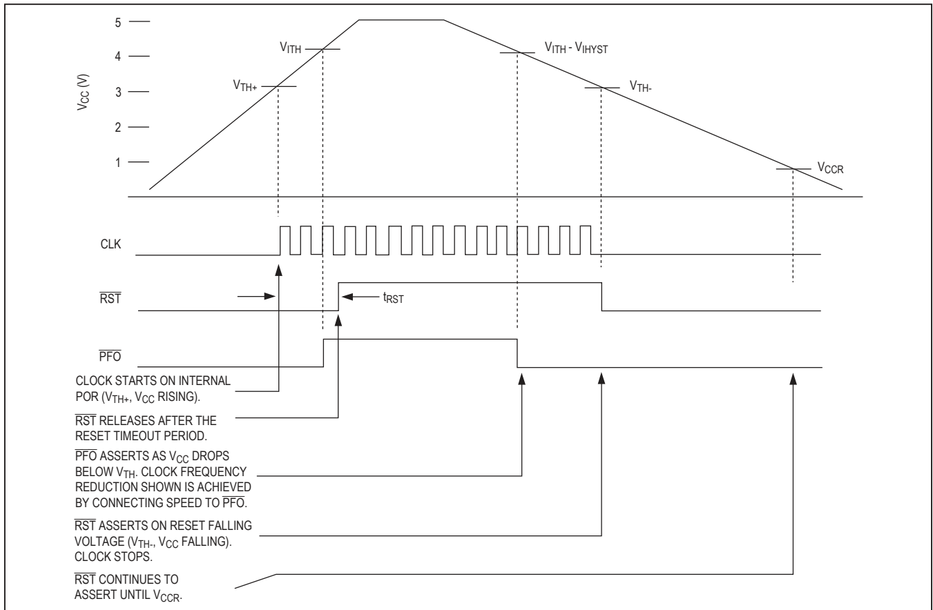
Figure 1. RST/\overline{RST} and \overline{PFO} Behavior During Power-Up and Brownout
