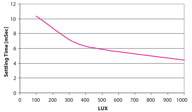
Figure 9. Average Settling Time vs Lux at Vcc=3V
