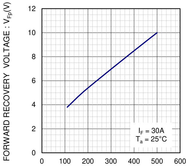
RATE OF CHANGE OF CURRENT : di/dt(A/μs) di/dt-V Fp CHARACTERISTICS
