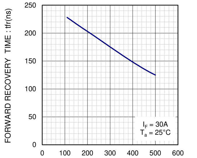
RATE OF CHANGE OF CURRENT : di/dt(A/μs) di/dt-t fr CHARACTERISTICS
