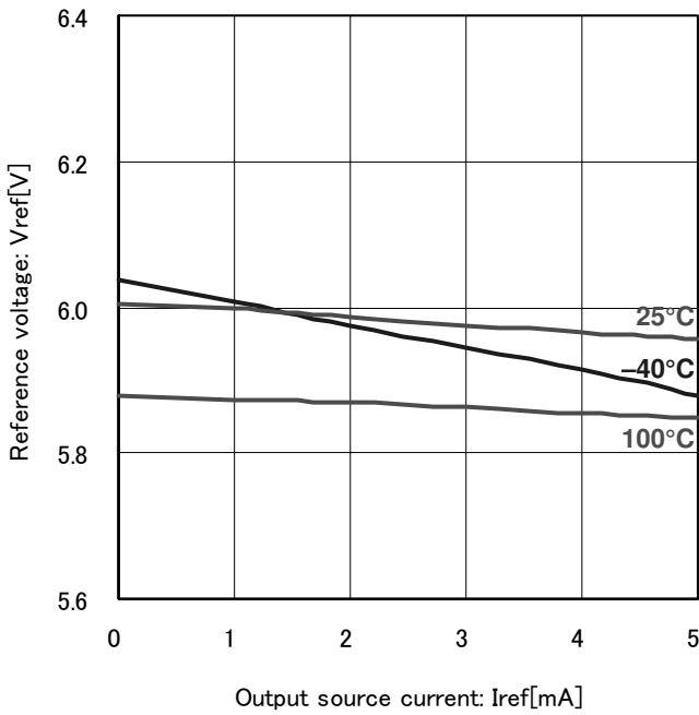
Fig.19 Reference voltage current ability ( V_{cc}=12V )
