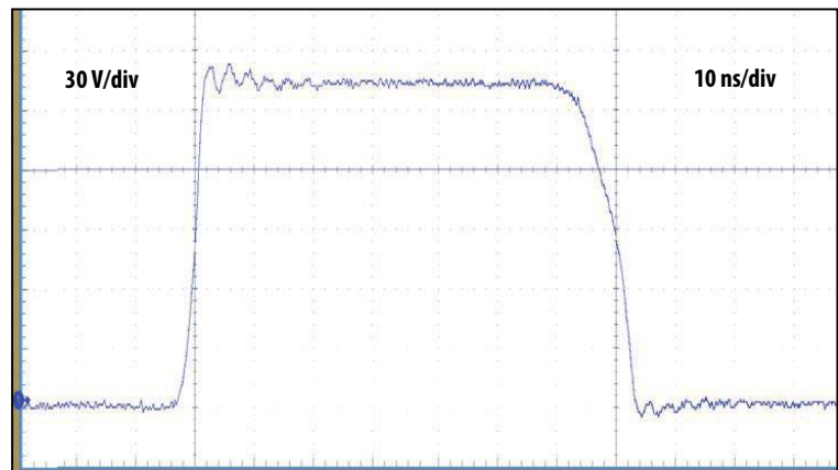
Figure 9: Typical switch-node waveform when operated as a buck converter
