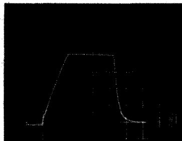
(A) SUPPLY TURN-ON AND TUNOFF CHARACTERISTICS
