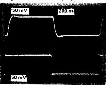
(A) SMALL SIGNAL RESPONSE 50mV/Div and 200ns/Div Top Trace: Output; 50mV/Div and 200ns/Div Bottom Trace: Input; 50mV/Div and 200ns/Div
