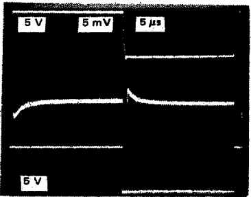
(B) INPUT-OUTPUT DIFFERENCE SIGNAL SHOWING SETTLING TIME (measurement made with Tektronix 7A13 differential amplifier) Top Trace: Output Signal; 5V/Div and 5μs/Div Center Trace: Difference Signal; 5mV/Div and 5μs/Div Bottom Trace: Input Signal; 5V/Div and 5μs/Div
