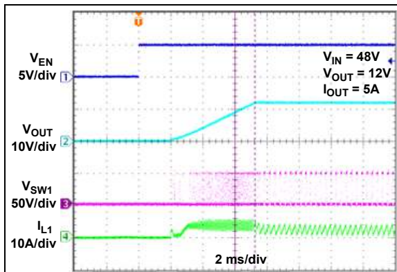
FIGURE 2-20: Soft Start with Enable ( V_{OUT} = 12V , I_{OUT} = 5A ).
