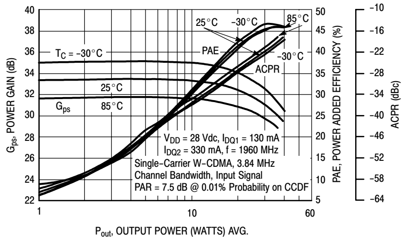
Figure 10. Single-Carrier W-CDMA Power Gain, Power Added Efficiency and ACPR versus Output Power
