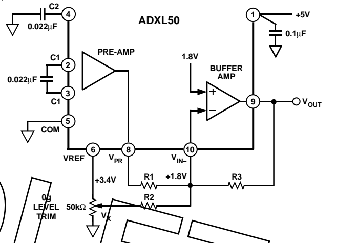
Figure 20. ADXL50 Circuit Using the Buffer Amplifier to Set the Output Scaling and 0 g Offset Level
