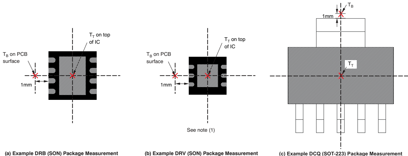
Figure 38. Measuring Points for T_T and T_B
