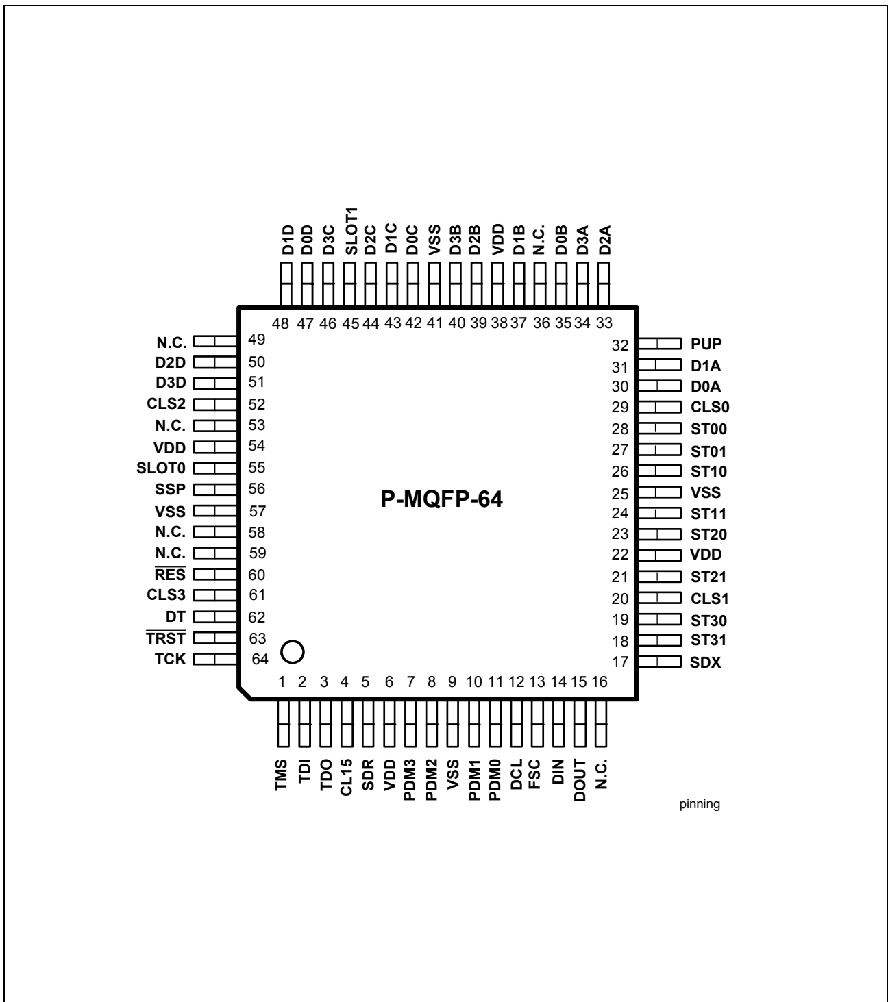
Figure 6 Pin Configuration
