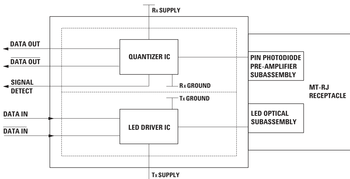
Figure 1. Block Diagram.
